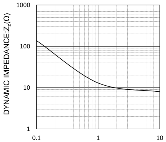
ZENER CURRENT: I_z (mA) I_z - Z_z CHARACTERISTICS
