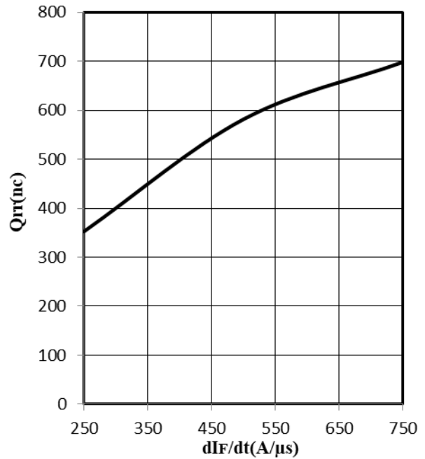
Fig 20. Typical Q rr as a function of dI F /dt
