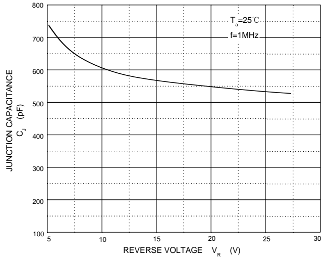
Capacitance Characteristics
